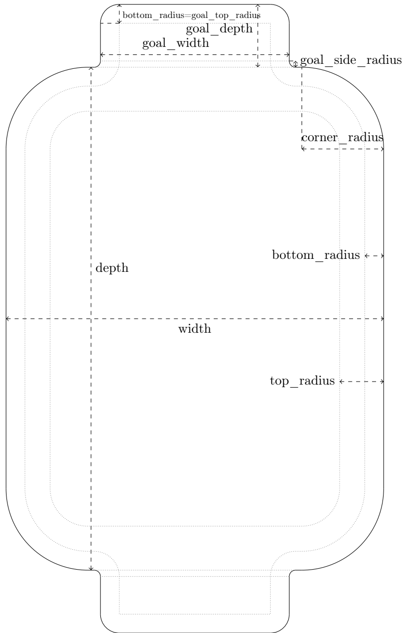
Figure 1.1: Top-down view
